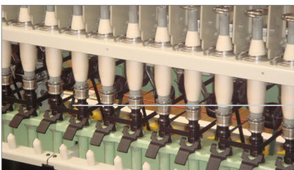
細紗機錠帶 VISBELT VS-5
