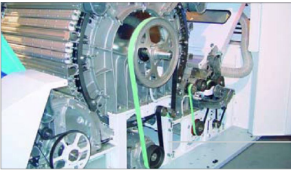
梳棉機傳動平皮帶 VISBELT S-25
